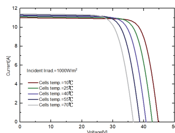
I-V Curves of SPP370QHES at different cell temperature
